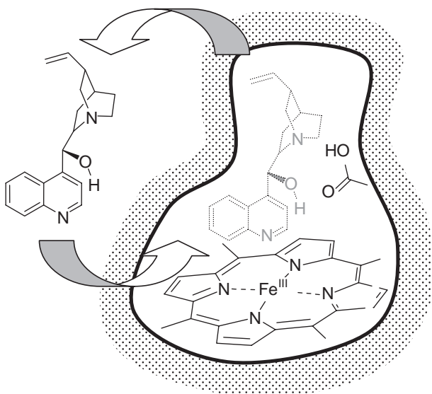
Fig. 1. Schematic representation of molecular imprinting of CD with the cooperative use of MAA and 2 as the functional monomers.
