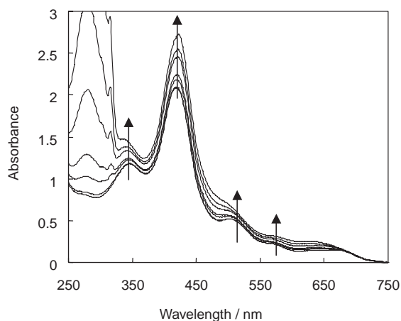
Fig. 4. UV-vis spectra of IP(P1M6) with various concentrations of CD (from bottom to top: 0, 10, 50, 100, 250, 500, and 1000 \mu\text{M} in \text{CH}_2\text{Cl}_2 , respectively).
