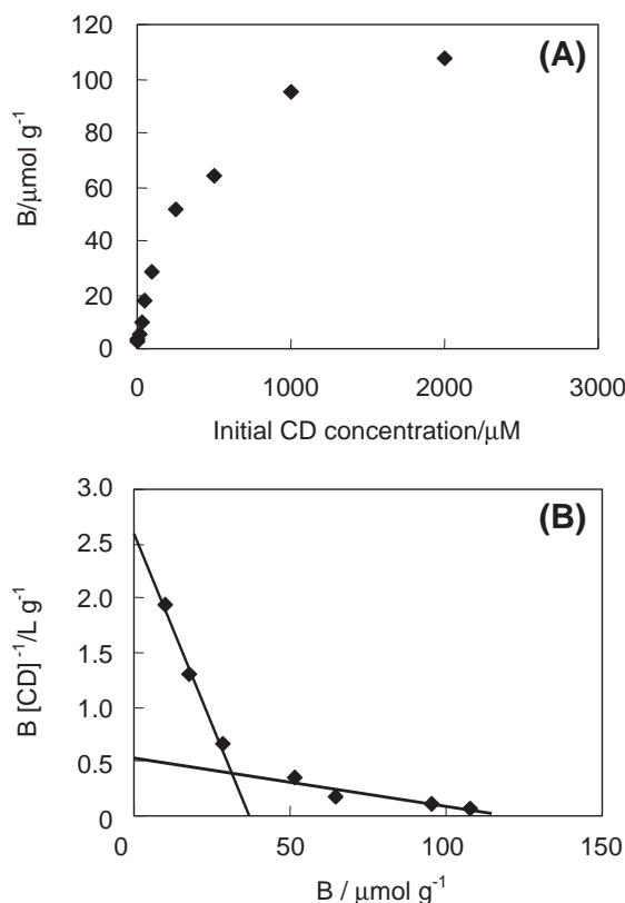
Fig. 3. Typical binding isotherm (A) and Scatchard plot (B) of IP(P1).
