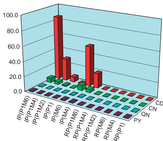
Fig. 2. Retention factors ( k' ) on the polymers prepared. A mixture of \text{CH}_2\text{Cl}_2 /acetic acid (99:1, v/v) was used as the eluent at 1.0 mL/min, and the detection was carried out at 280 nm. Retention factors ( k' ) were calculated by an equation, k' = (t_R - t_0)/t_0 , where t_R is the retention time of a sample and t_0 is the retention time of a marker. CD: cinchonidine, CN: cinchonine, QN: quinoline, PY: pyridine.
